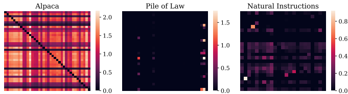
Figure 2. Heatmaps of adjacency matrices we compute for skill graphs for Alpaca, Pile of Law, and Natural Instructions (see Appendix D.2 for descriptions of how they were constructed and larger versions).
