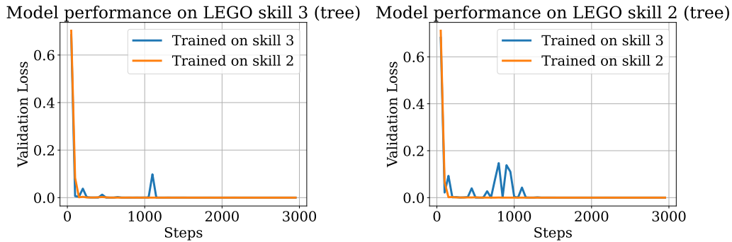
Figure 16. Performance on LEGO skill 2 and 3 when training on skills 2 and 3. The reasoning pattern is a tree rather than a chain over k = 4 variables. Skills 2 and 3 are at the same “depth” in the graph and both depend on skill 1, so there is positive influence between the skills despite there being no edge between 2 and 3 in the LEGO reasoning graph.
