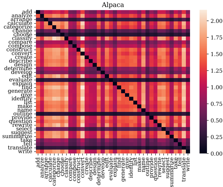
Figure 7. Alpaca heatmap where i, j th entry is \max(0, \delta_j^i) (the change in loss on s_j after training on s_i for 150 steps). Diagonal entries are set to 0 for clearer visualization.
