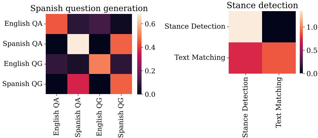
Figure 12. Spanish question generation and stance detection heatmaps where i, j th entry is \max(0, \delta_j^i) (the change in loss on s_j after training on s_i for 100 steps).
