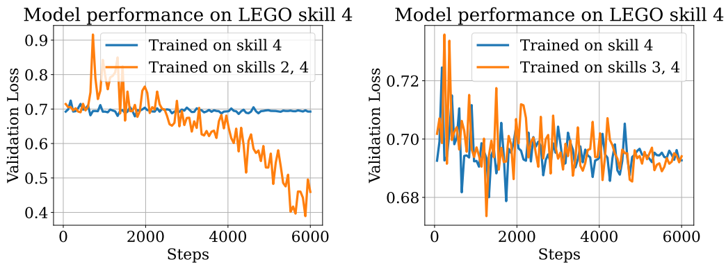
Figure 15. Performance on LEGO skill 4 when training on skill 4, skills 2 and 4, and skills 3 and 4. Even though skill 3 and skill 4 share an edge in the LEGO synthetic’s underlying reasoning chain (i.e. a model predicting correct for the fourth variable is one extra step beyond predicting correct for the third variable), we find that training on skills 2 and 4 helps improve performance on skill 4 more.
