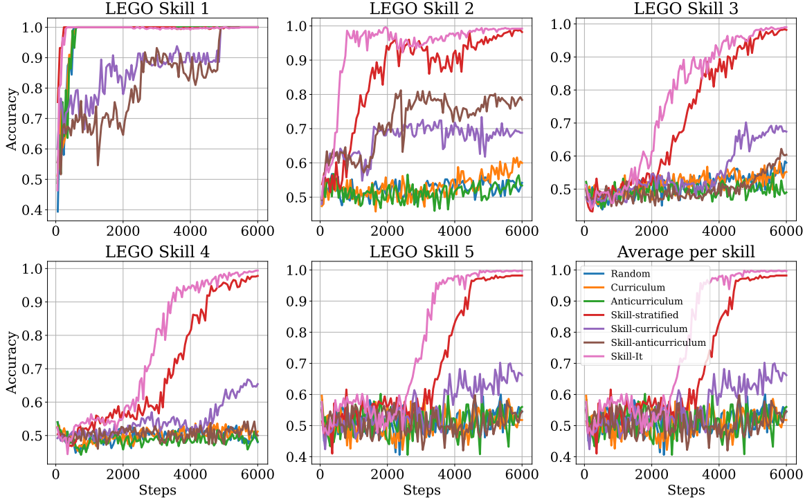
Figure 18. Accuracy of SKILL-IT on each skill (binary classification) on the LEGO synthetic in the continual pre-training setting. SKILL-IT attains higher accuracy more quickly than baselines that both do and do not utilize the notion of skills.
