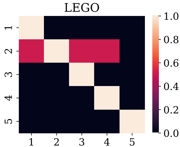
Figure 9. LEGO heatmap with k = 5 where i, j th entry is set to 0.5 if the number of steps needed to reach 0.01 loss on skill j when training on a balanced mixture of skills i and j is less than when training on skill j only.
