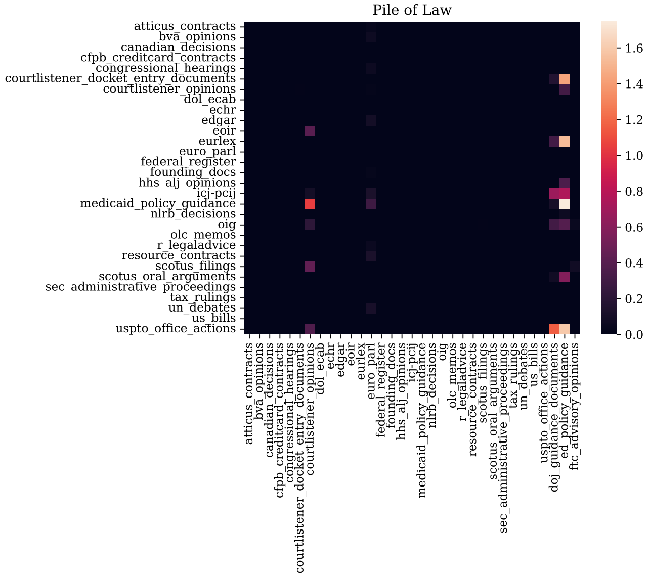
Figure 8. Pile of Law heatmap where i, j th entry is \max(0, \delta_j^i) (the change in loss on s_j after training on s_i for 150 steps). Diagonal entries are set to 0 for clearer visualization.
