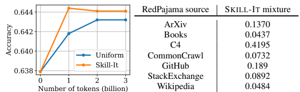
Figure 6. Left: Accuracy on LM Evaluation Harness for continual pre-training of a 3B parameter model using SKILL-IT on the RedPajama dataset. We achieve higher accuracy at 1B additional tokens than uniform at 3B tokens. Right: SKILL-IT mixture over RedPajama sources.
