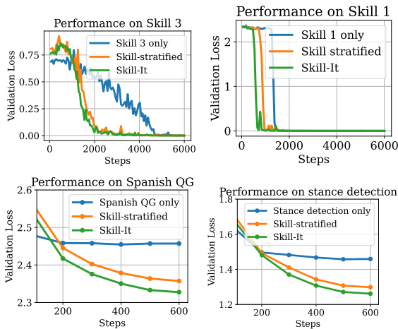
Figure 5. Performance of SKILL-IT in the fine-tuning setting (learning a target skill using the ordered training skill set) on LEGO, addition, and NL.
