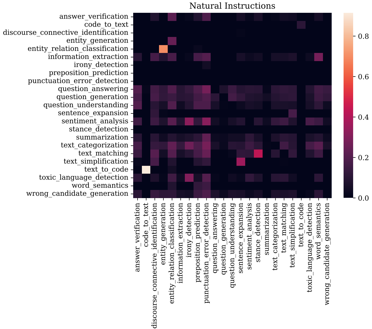
Figure 11. Natural Instructions heatmap where i, j th entry is \max(0, \delta_j^i) (the change in loss on s_j after training on s_i for 100 steps). Diagonal entries are set to 0 for clearer visualization.
