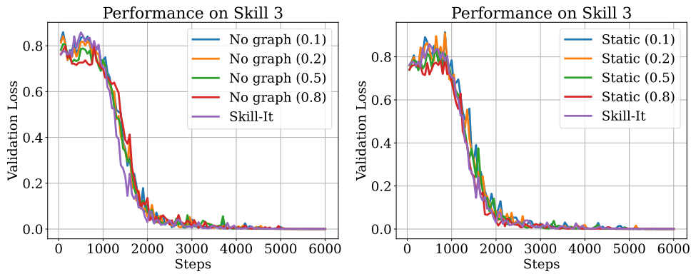
Figure 30. Comparison of SKILL-IT versus using no graph (left) and static data selection (right) with \eta = 0.1, 0.2, 0.5, 0.8 on the LEGO fine-tuning experiment. All approaches have roughly the same loss trajectories, but SKILL-IT is slightly lower than using no graph.
