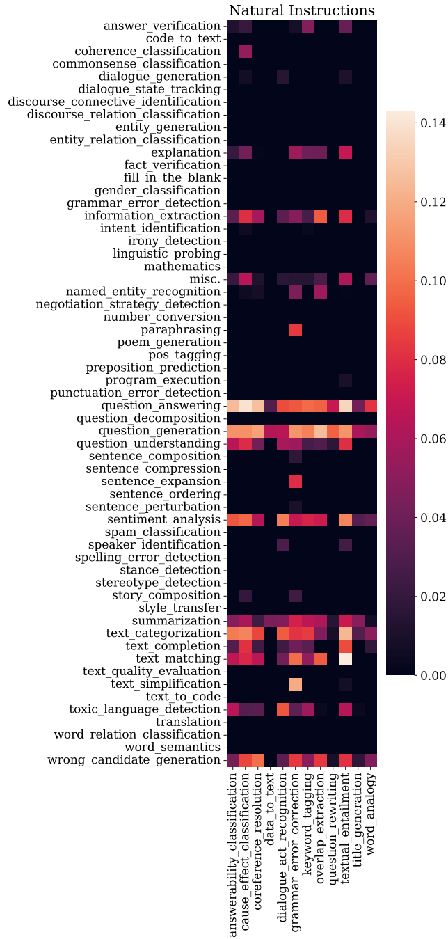
Figure 13. Natural Instructions heatmap for out-of-domain setting where rows are for the training skills and columns are for the evaluation skills. The i, j th entry is \max(0, \delta_j^i) (the change in loss on s_j after training on s_i for 100 steps).
