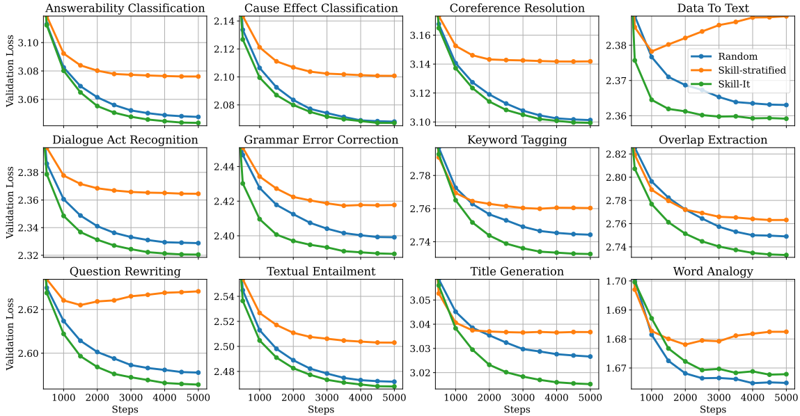
Figure 19. Performance of SKILL-IT in the out-of-domain setting for the NI test task split. SKILL-IT uses the graph between the train and evaluation skills to produce an online mixture on the training dataset.
