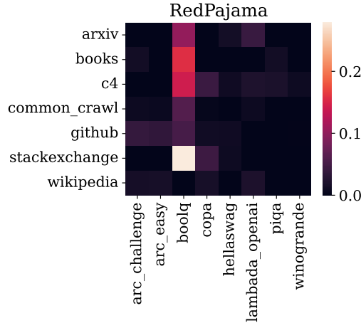
Figure 14. RedPajama heatmap for out-of-domain setting where rows are for the training skills and columns are for the evaluation skills. The i, j th entry is \max(0, \delta_j^i) (the change in perplexity on s_j after training on s_i for 1B tokens).
