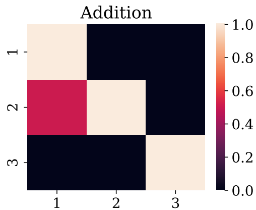
Figure 10. Addition heatmap with k = 3 where i, j th entry is set to 0.5 if the number of steps needed to reach 0.01 loss on skill j when training on a balanced mixture of skills i and j is less than when training on skill j only.
